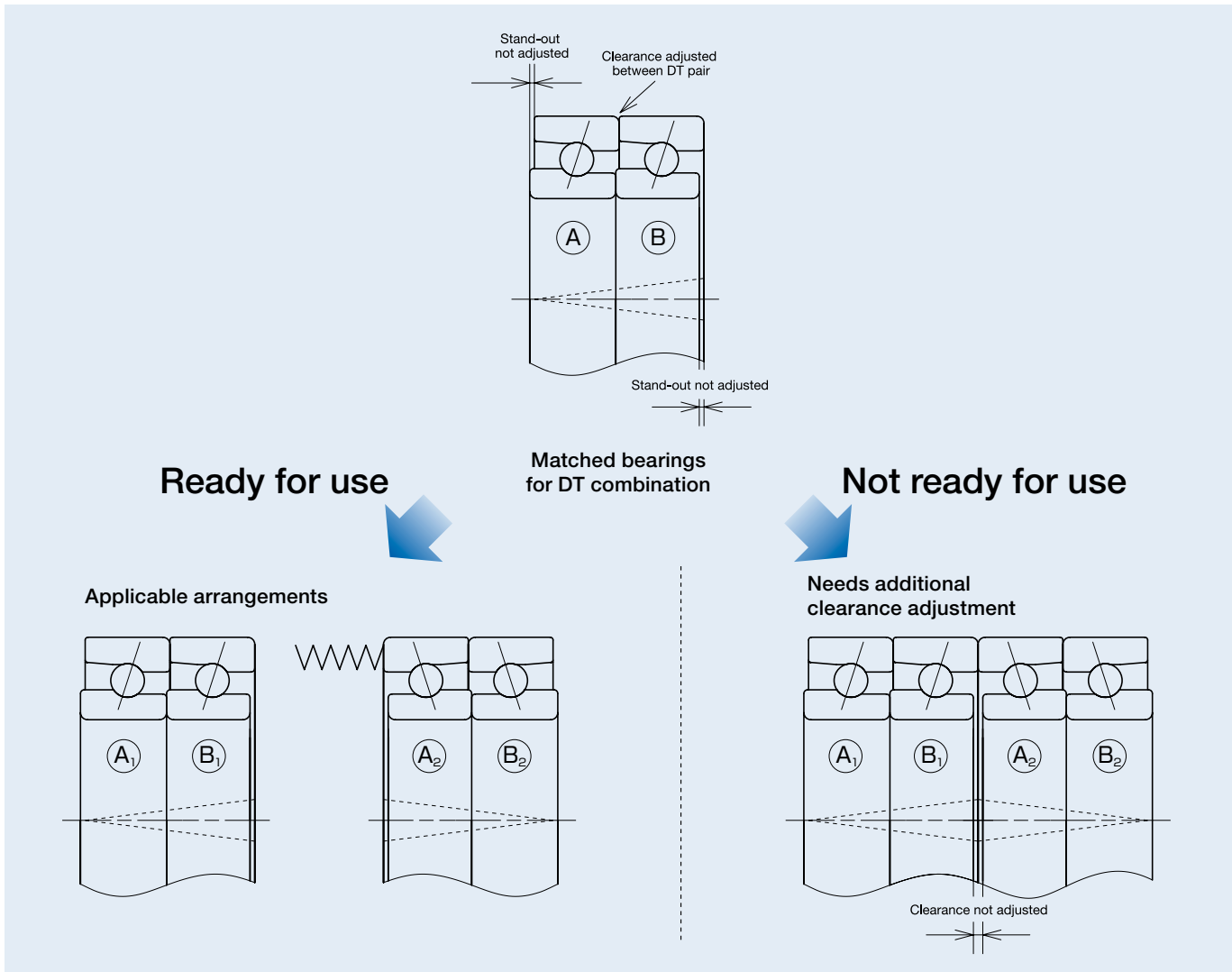
Fig. 3.7 DT Combination
