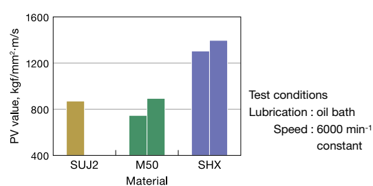
Oil Bath Seizure Limit Test (4 Balls Test)
