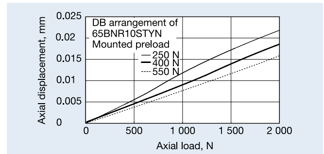
Fig. 1.36 Relationship between Axial Displacement and Preload
