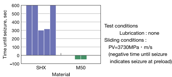
Dry Seizure Limit Test (4 Balls Test)
