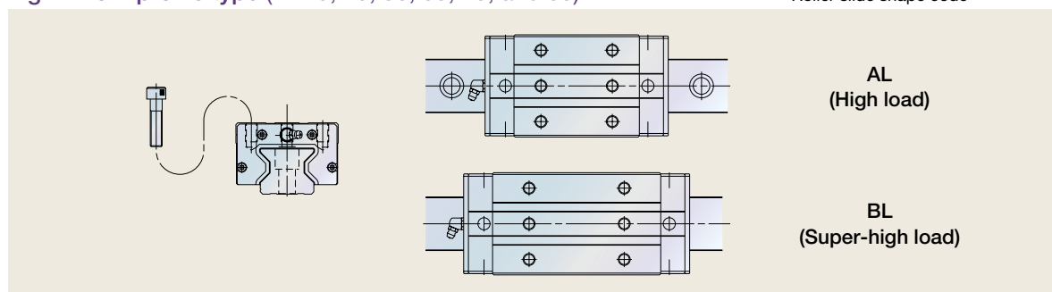
Fig. 3 Flange type (RA15, 20, 25, 30, 35, 45, 55, and 65)
