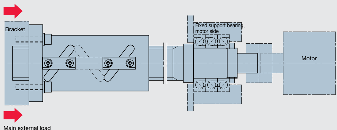
HTF-SRC, HTF-ASRC, HTF type of recommended mounting direction
